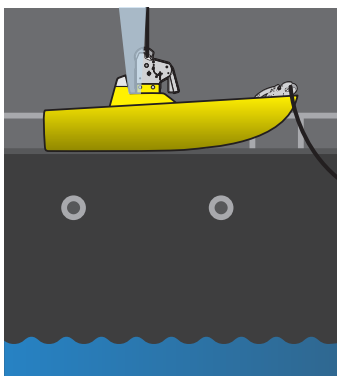
1. Hook closed
